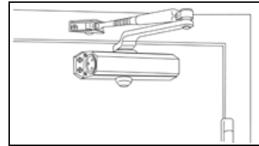
Regular Arm Installation
