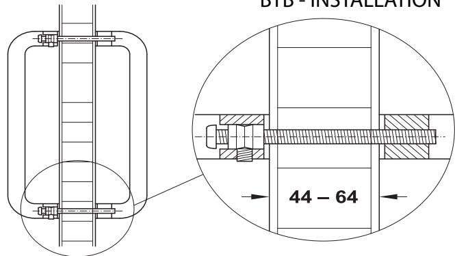
BTB - INSTALLATION
